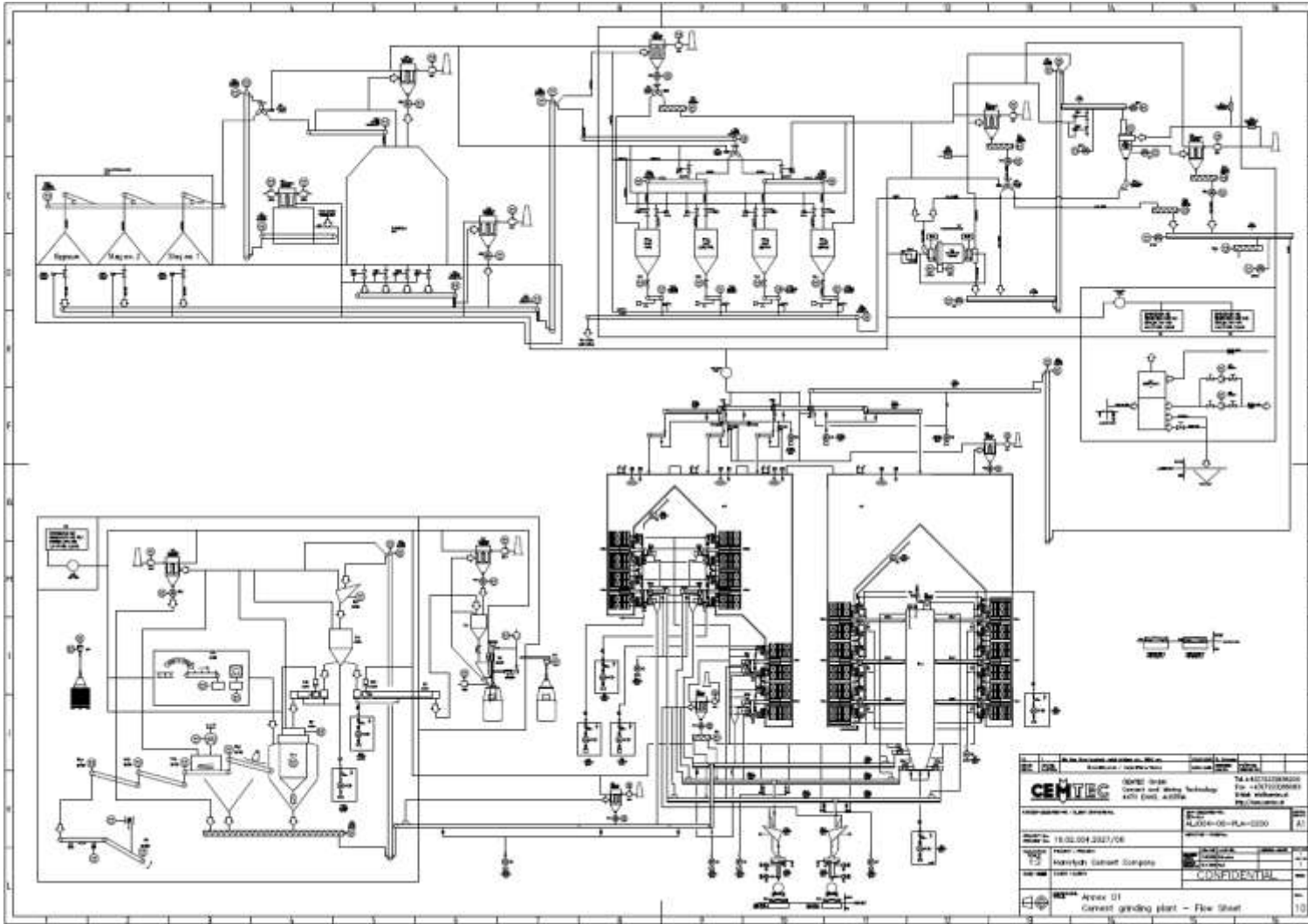
Flow diagram - cement grinding plant – 115 tph
